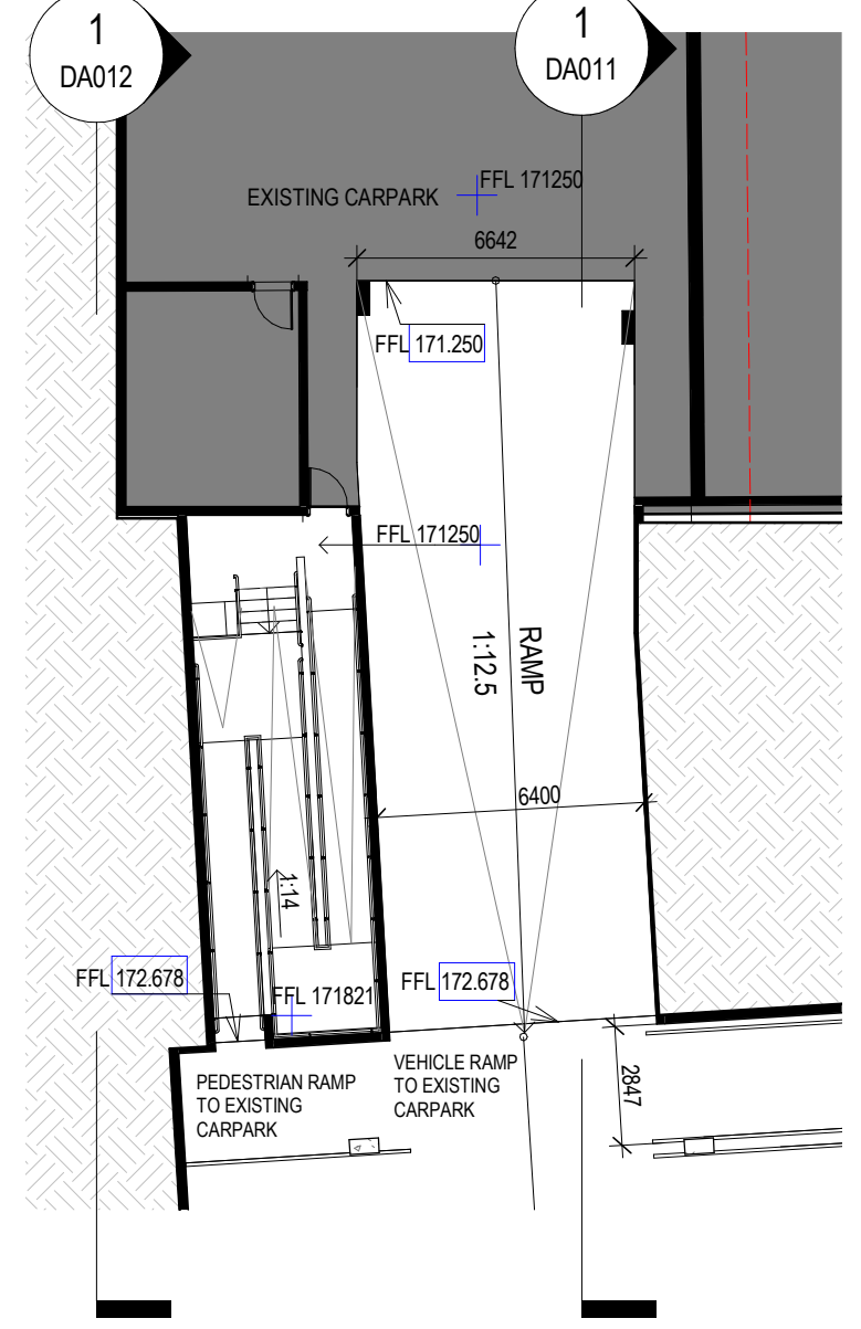
2 BASEMENT FLOOR PLAN SCALE 1 : 200
